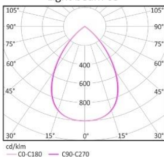
Light beam 65°
